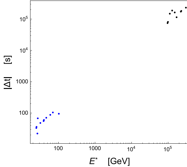
Fig. 1. Values of |\Delta t| versus E^* for the IceCube GRB-neutrino candidates discussed in Refs. 10,12 (black points) and for the GRB photons discussed in Refs. 12,15 (blue points). The photon points in figure also factor in the result of a one-parameter fit estimating the average magnitude of intrinsic time lags (details in Refs. 12,15 ).
